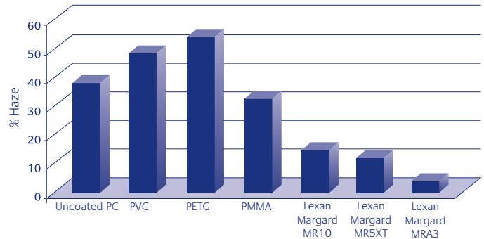
Figure 5 Taber abrasion ASTM D1044 test at 500 cycles
